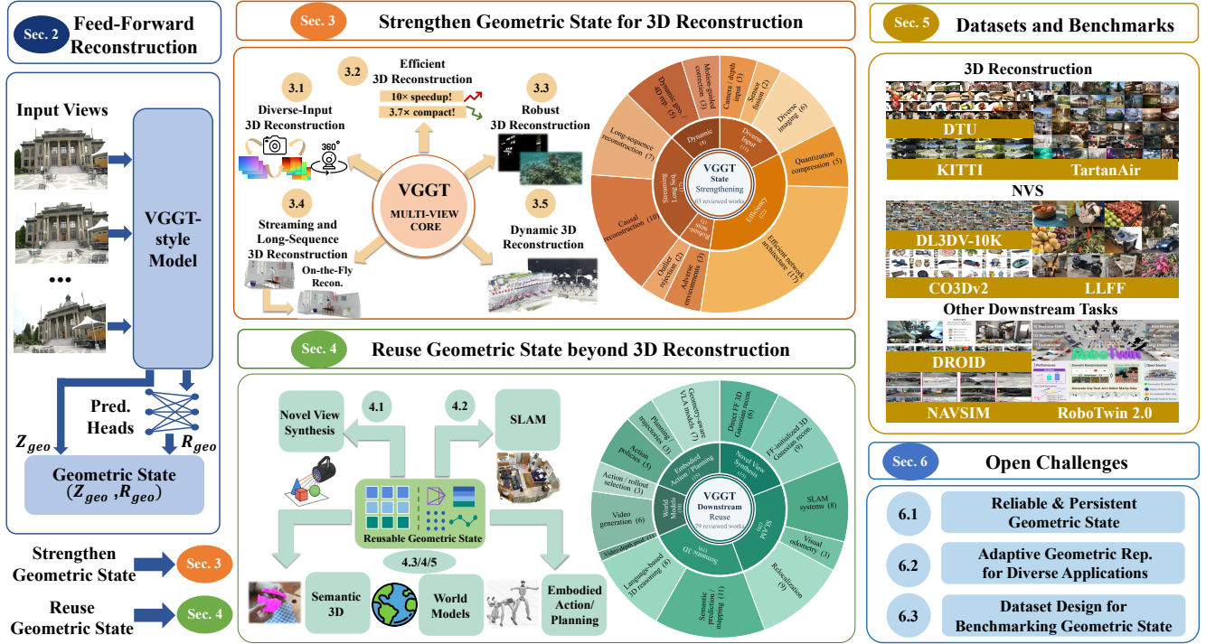
Figure 1: Overview of the survey organization. Feed-forward reconstruction produces a geometric state containing multi-view geometry latent features Z_{geo} and structured geometric outputs R_{geo} . State-strengthening methods improve how this state is formed, computed, made robust, retained over streams, or extended to dynamic scenes. Downstream methods reuse geometric state for novel-view synthesis, SLAM, semantic 3D scene understanding, geometry-aware world models, and embodied action and planning. Datasets and evaluation targets assess the reviewed methods, and the open challenges concern reliable and persistent state, adaptive representations, and dataset design for benchmarking geometric state. Numbers in parentheses indicate the number of reviewed works in each category or subcategory.
