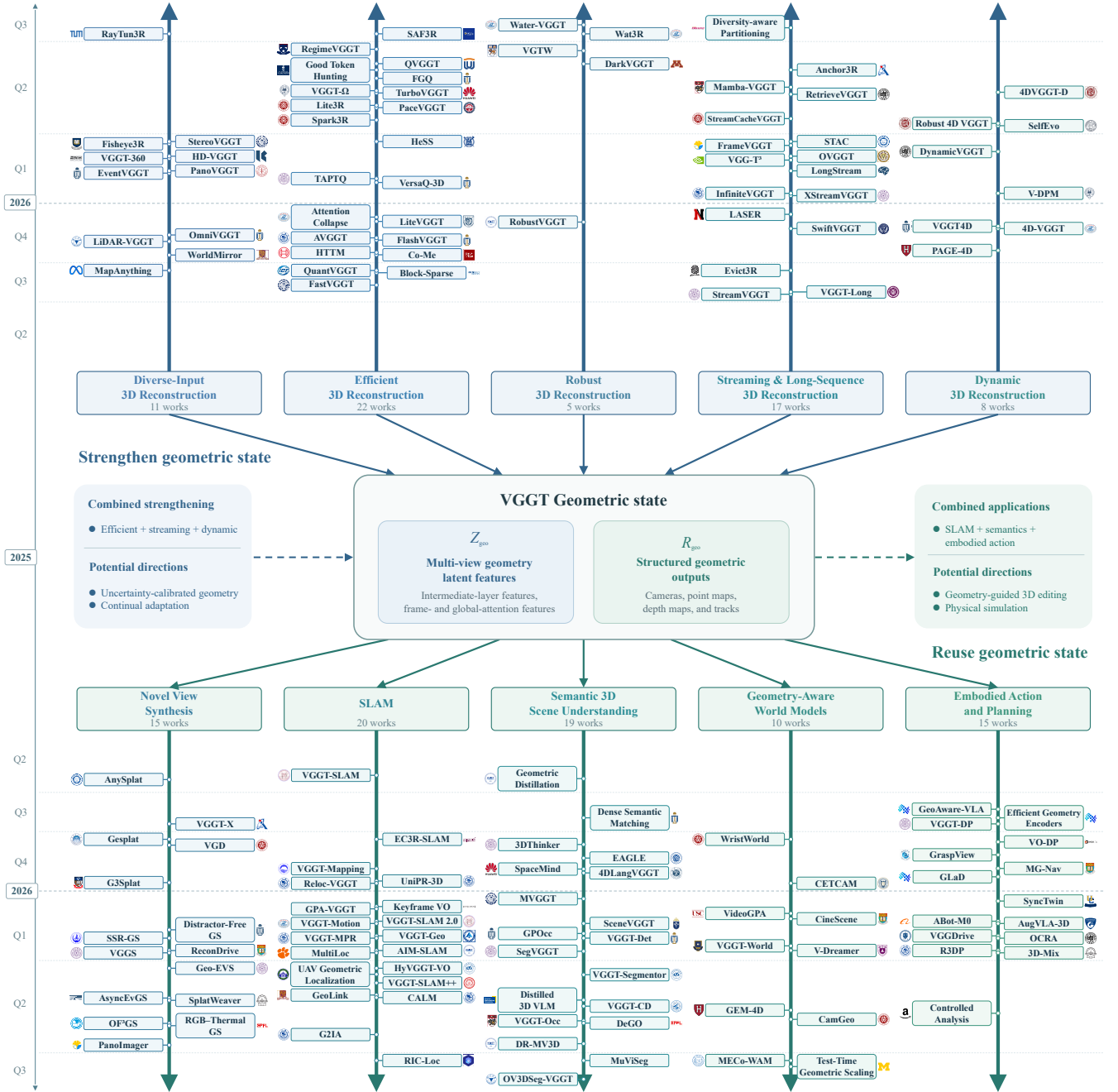
Figure 3: Development of the VGGT [WCK*25] lineage around geometric state. The center contains multi-view geometry latent features Z_{\text{geo}} and structured geometric outputs R_{\text{geo}} . The 5 upper branches organize geometric-state strengthening methods, and the 5 lower branches organize downstream applications. Methods follow chronological order outward from the center, with years and quarters marked on the left. The side panels illustrate combinations of strengthening directions and applications, together with potential directions.
