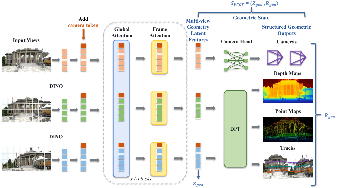
Figure 2: VGGT [WCK*25] architecture. Input images are converted into tokens and augmented with camera and register tokens. Alternating frame-wise and global attention produces the multi-view geometry latent features \mathcal{Z}_{\text{geo}} . Prediction heads decode cameras, depth maps, point maps, and tracks as the structured geometric outputs \mathcal{R}_{\text{geo}} .
