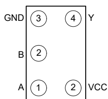
Figure 4-3. YZP Package, 5-Pin DSBGA (Top View)
