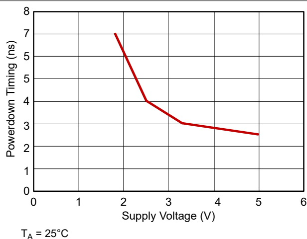
Figure 5-2. Powerdown Timing vs Supply Voltage
