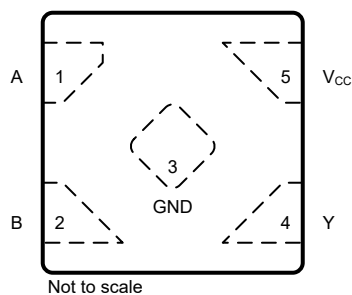
Figure 4-2. DPW Package, 5-Pin X2SON (Top View)
