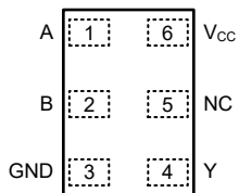
Figure 4-4. DRY or DSF Package, 6-Pin SON (Top View)
