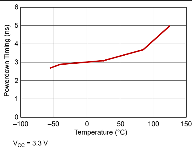
Figure 5-1. Powerdown Timing vs Temperature
