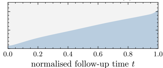
(b) Random effects, combined cloud
