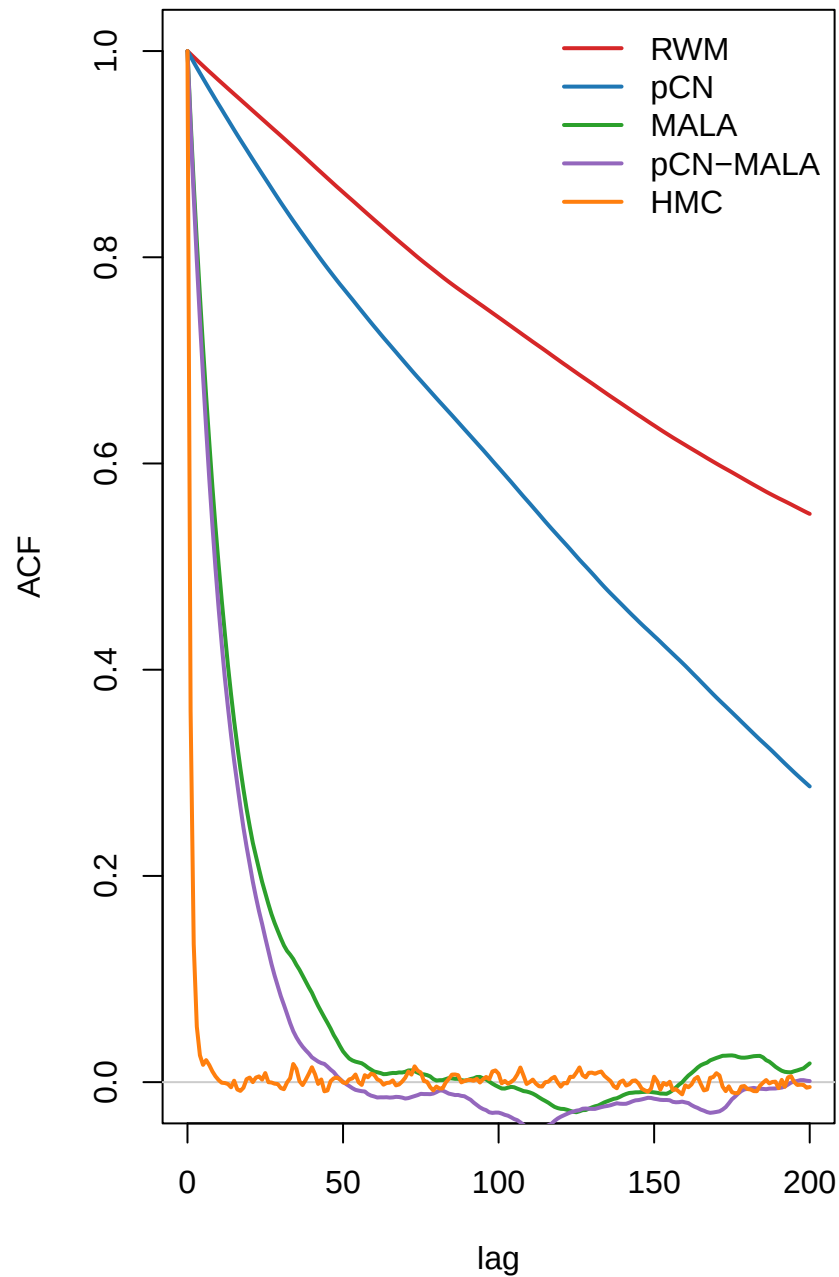
ACF of worst-mixing u-coordinate
