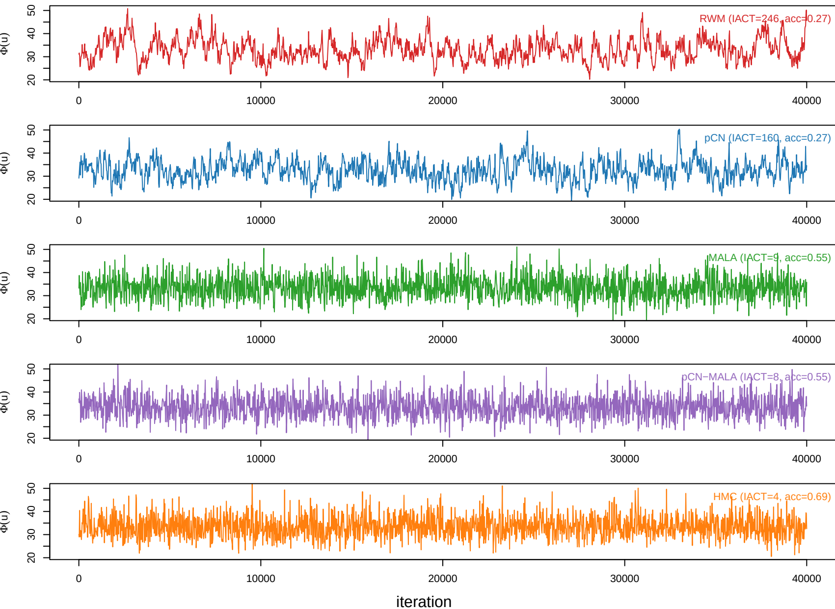
Trace of the ABC potential \Phi(u) = 1/2||Au-y||^2/\epsilon^2
