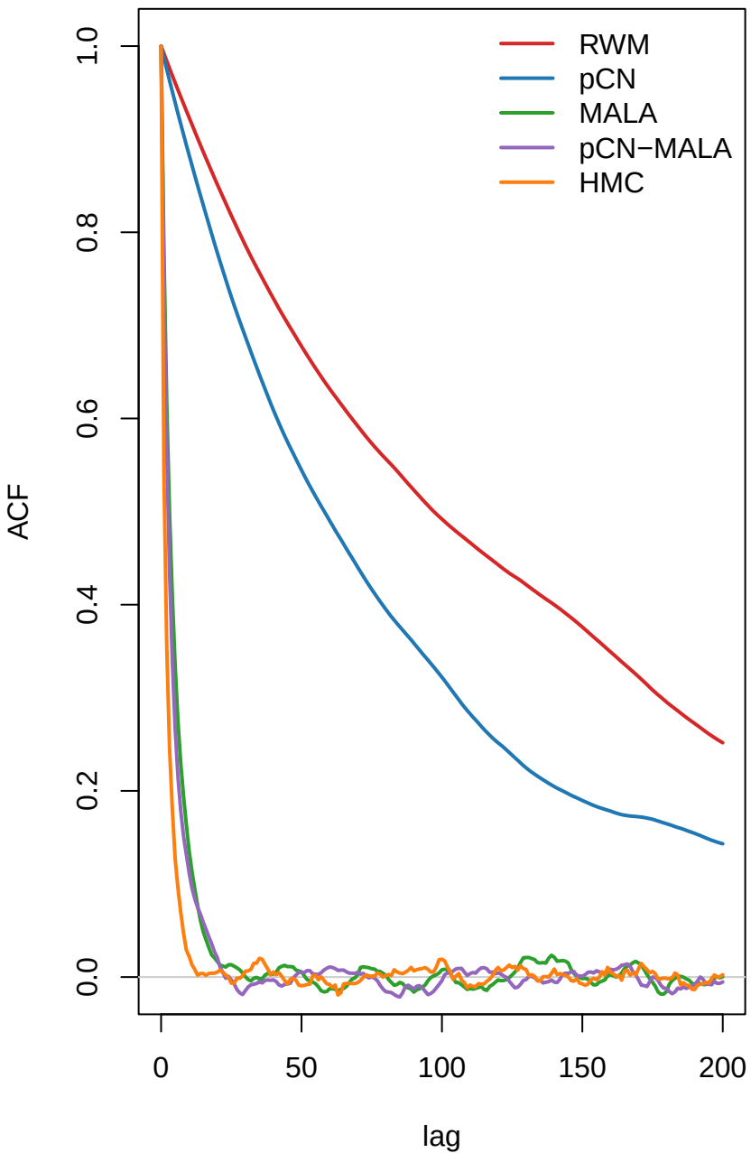
ACF of \Phi(u)
