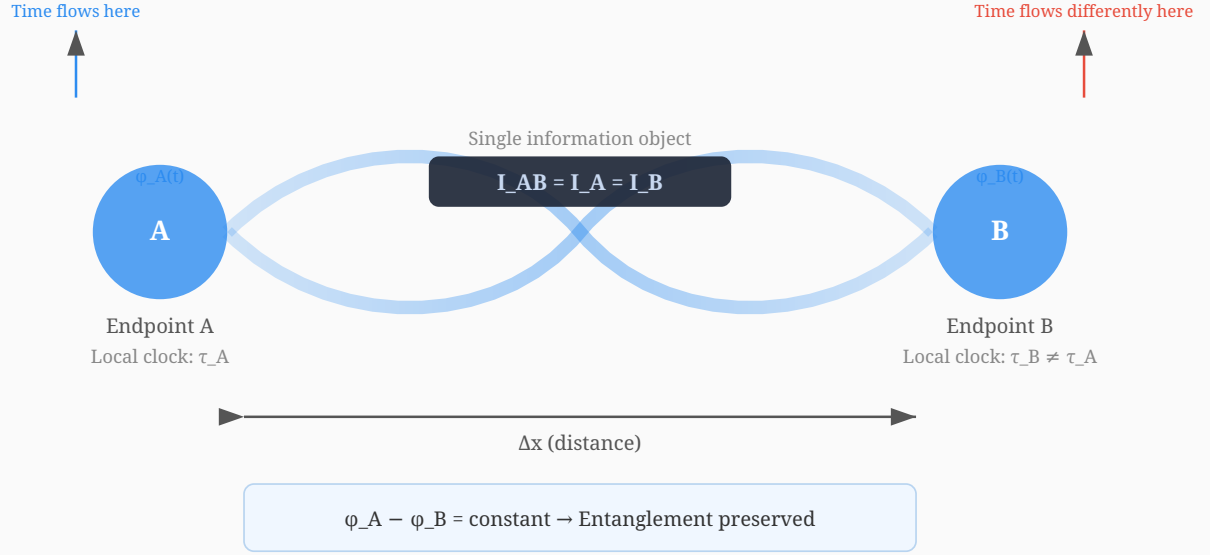
Figure 1: Entanglement is a single information object \mathcal{I}_{AB} spanning two endpoints A and B with different local time densities ( \tau_A \neq \tau_B ). The phase difference (\phi_A - \phi_B) remains constant, preserving entanglement.
