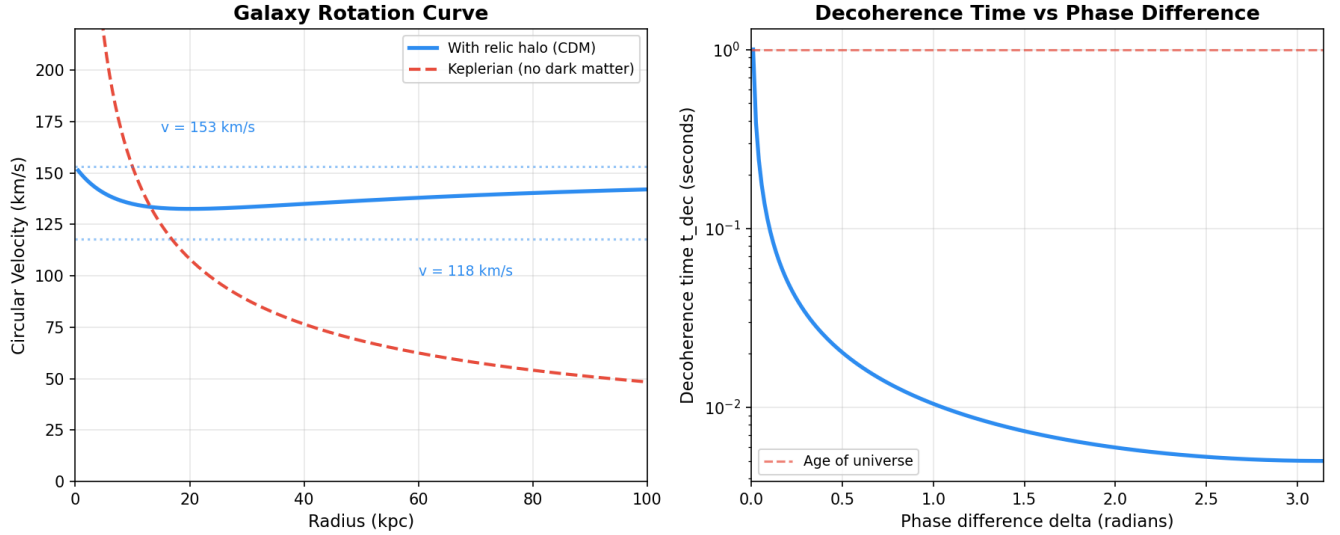
Figure 2: Figure 2: Right panel: Decoherence time \langle t_{\text{dec}} \rangle as a function of the phase difference \langle \delta \rangle between two endpoints. At \langle \delta = 0 \rangle (perfect coherence), \langle t_{\text{dec}} \rangle \rightarrow \infty . As \langle \delta \rangle increases, decoherence accelerates.
