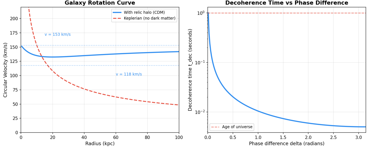
Figure 2: Figure 2: Right panel: Decoherence time (t_{\text{dec}}) as a function of the phase difference (\delta) between two endpoints. At (\delta = 0) (perfect coherence), (t_{\text{dec}} \rightarrow \infty) . As (\delta) increases, decoherence accelerates.
