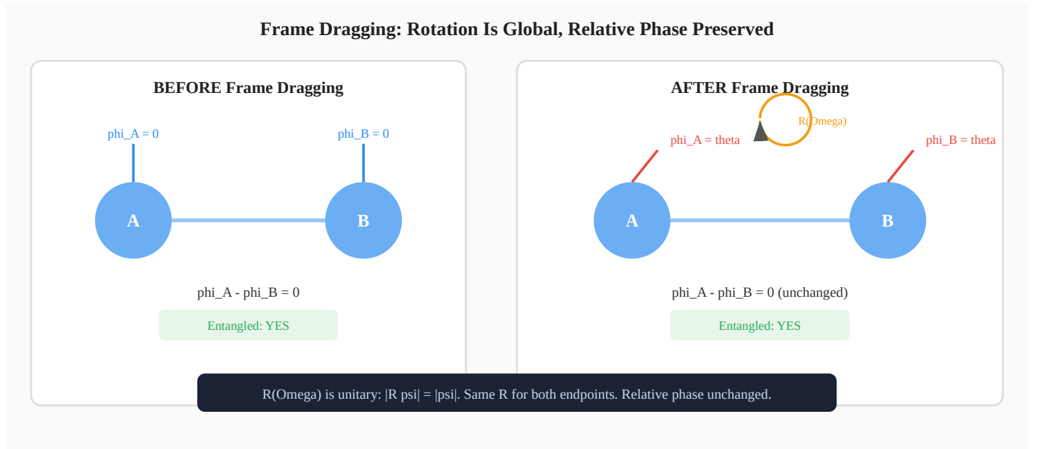
Figure 3: Frame dragging rotates both phases by the same amount R(\Omega) . The relative phase \phi_A - \phi_B is unchanged. Entanglement is preserved.
