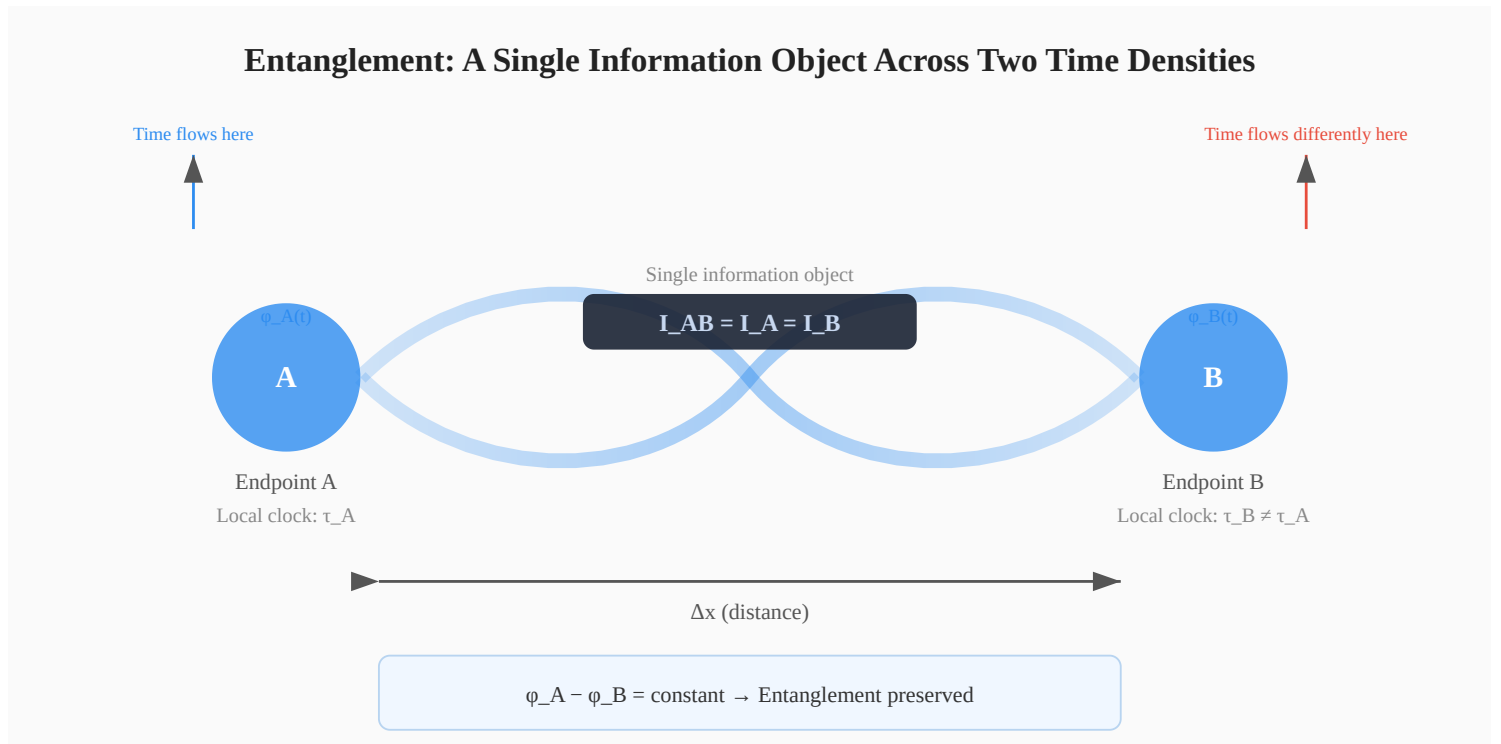
Figure 1: Entanglement is a single information object \mathcal{I}_{AB} spanning two endpoints A and B with different local time densities ( \tau_A \neq \tau_B ).
