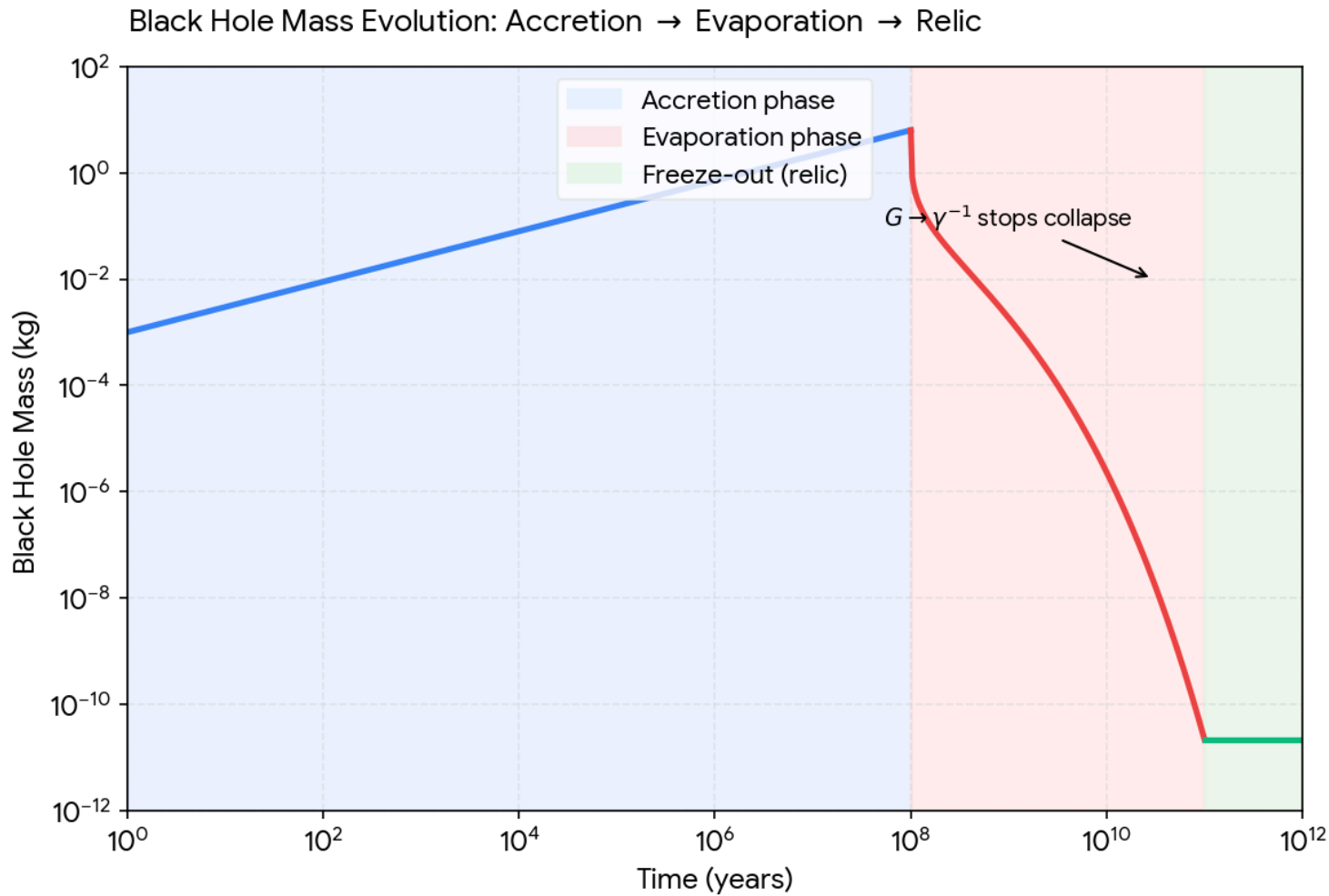
Figure 1: Black hole mass evolution across three phases. Accretion dominates at high mass, evaporation dominates at low mass, and the field-driven freeze-out mechanism halts collapse at M_{\text{relic}} > 0 , preserving information.
