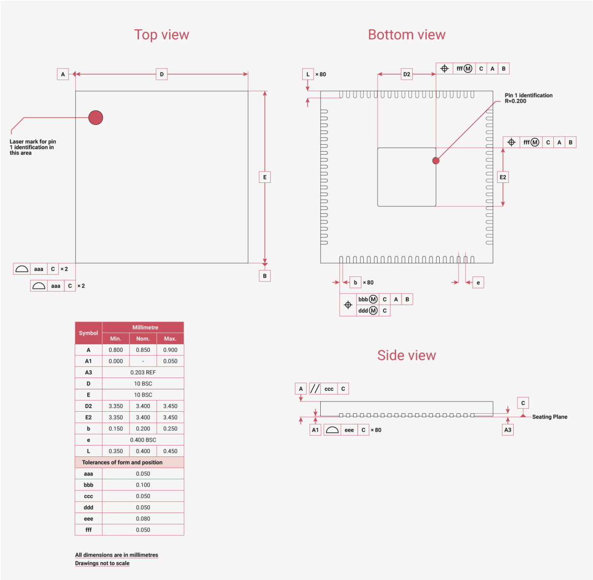
Figure 149. Top down view (left, top) and side view (right, bottom), along with bottom view (right, top) of the RP2350 QFN-80 package
