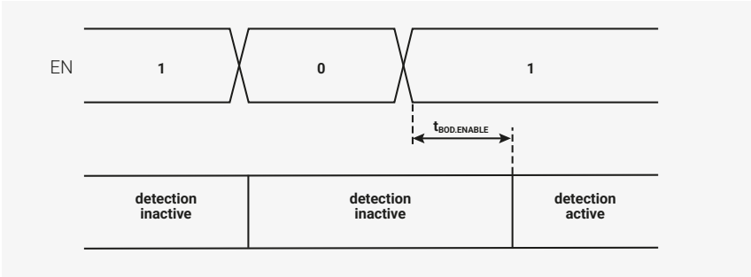
Figure 34. Disabling and enabling brownout detection
