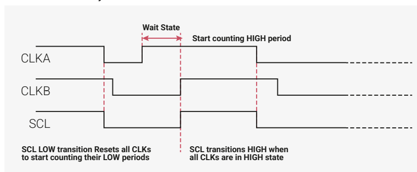
Multi-Master Clock Synchronisation
