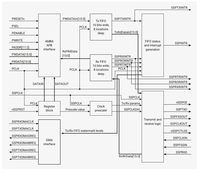
Figure 95. PrimeCell SSP block diagram. For clarity, does not show the test logic.
