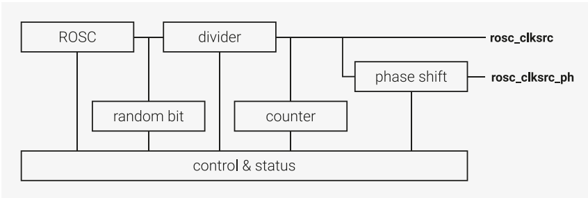
Figure 42. ROSC overview
