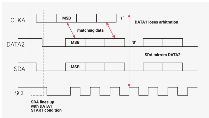
Multiple Master Arbitration
