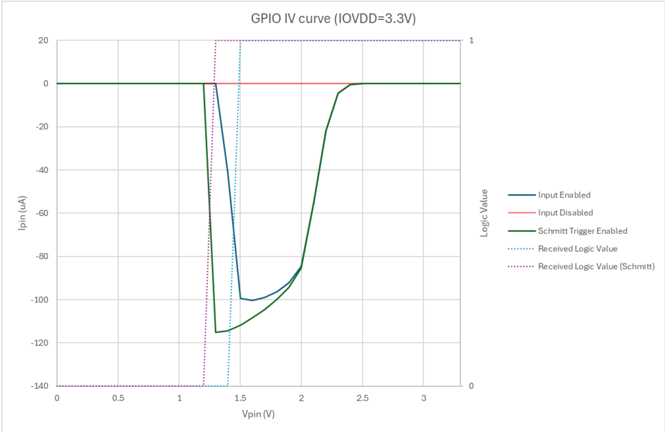
Figure 157. GPIO Pad leakage for IOVDD=3.3 V
