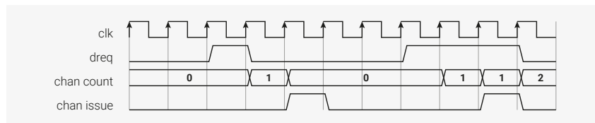
Figure 127. DREQ counting
