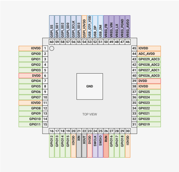
Figure 152. RP2350 Pinout for QFN-60 7×7mm
