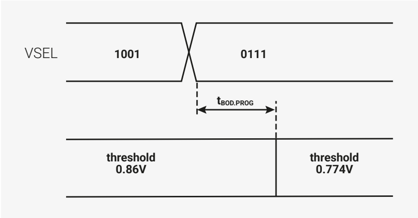
Figure 35. Adjusting the brownout detection threshold
