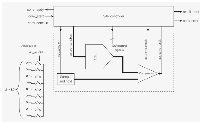
SAR ADC Block diagram QFN-80
