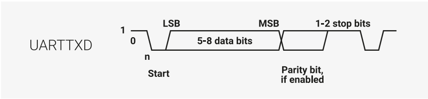
Figure 69. UART character frame.
