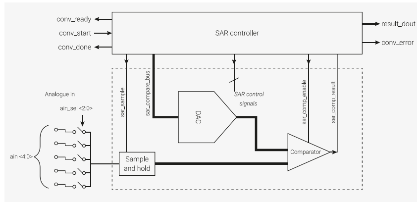
SAR ADC Block diagram QFN-60
