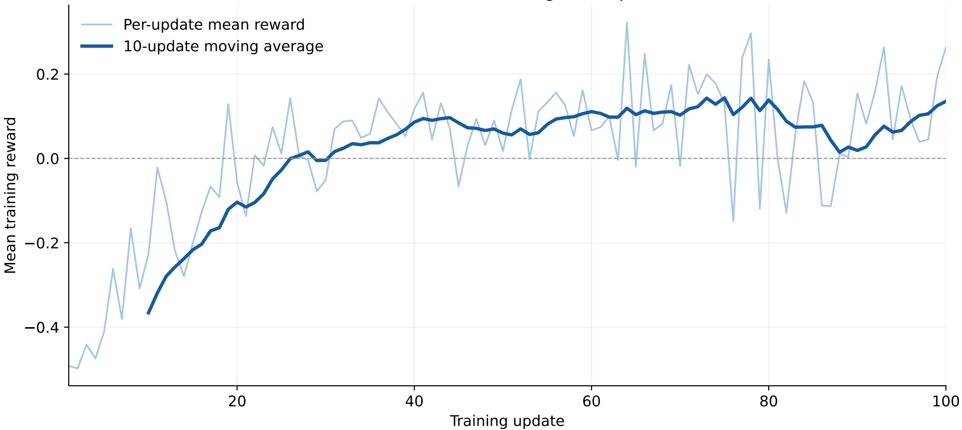
Baseline — DAPO training (100 updates)
