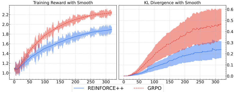
Figure 2: Comparison of smoothed Training Reward and KL Divergence. REINFORCE++ ( k = 1 ) achieves strong rewards with significantly more stable (lower) KL divergence, avoiding GRPO’s reward-hacking behavior.
