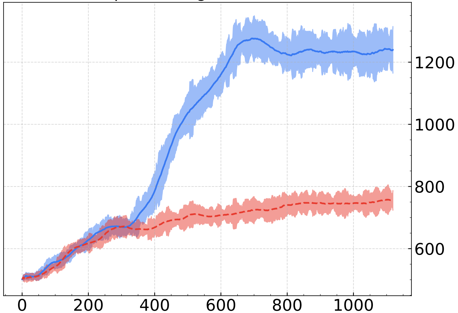
Response Length with Smooth
