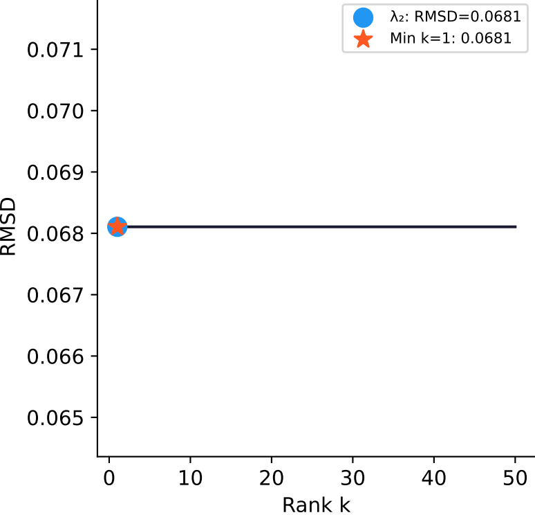
D. RMSD Landscape
