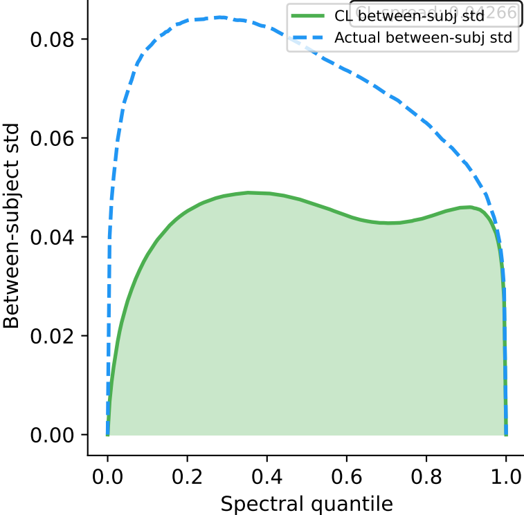
B. CL Convergence to Archetype
