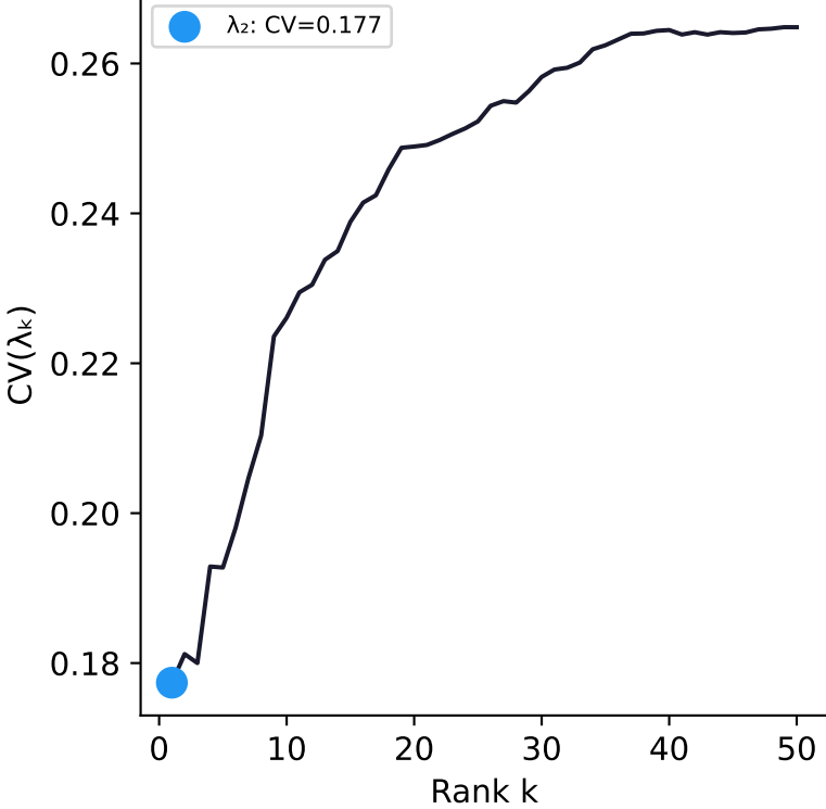
C. Eigenvalue Stability Profile
