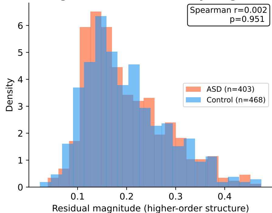
C. Higher-Order Structure by Diagnosis
