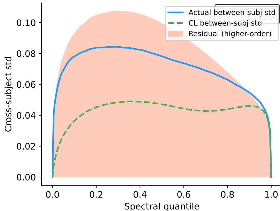
B. Variance Decomposition
