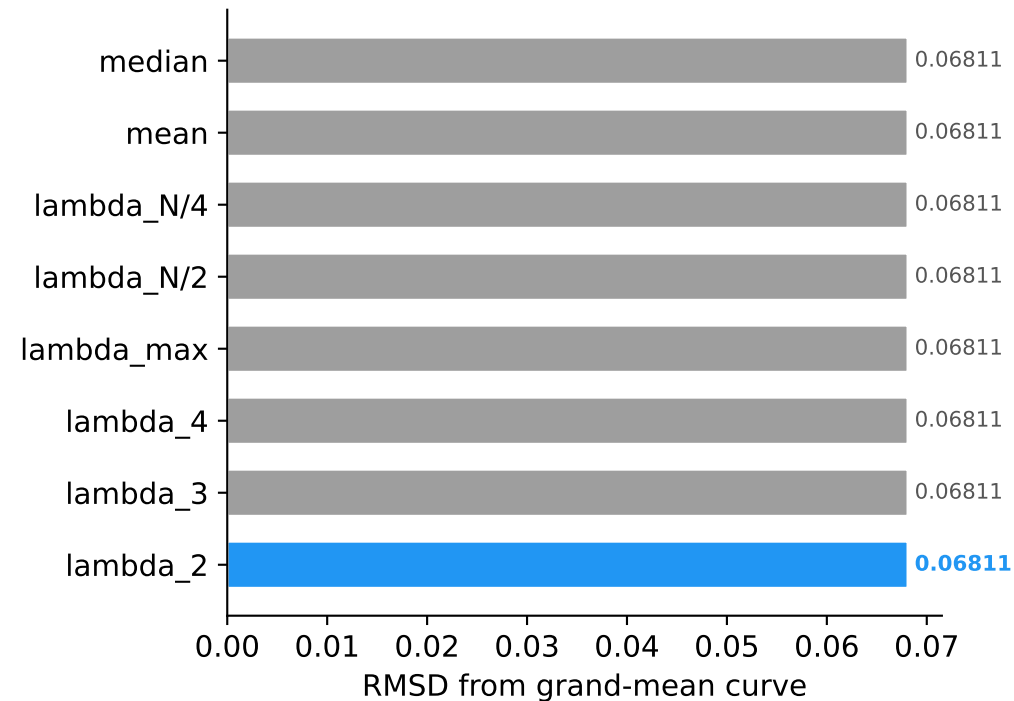
C. Named Candidate RMSD
