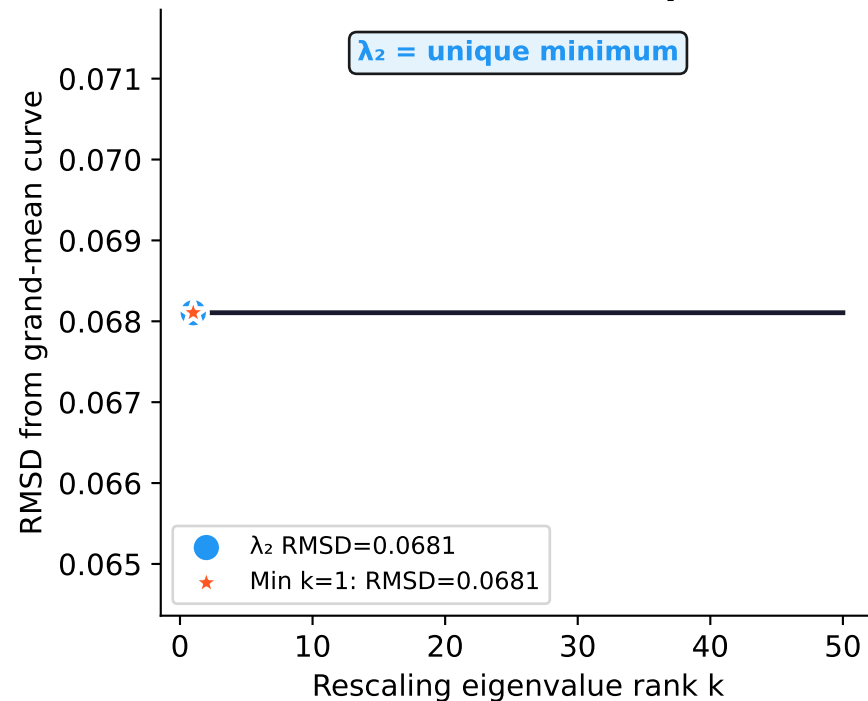
B. RMSD Landscape
