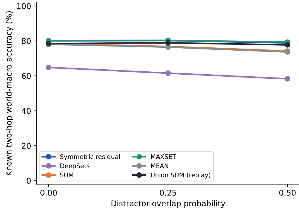
Equal-fit means across overlap
