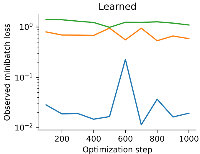
All registered fits; unsmoothed 100-step log samples (different phase objectives)
