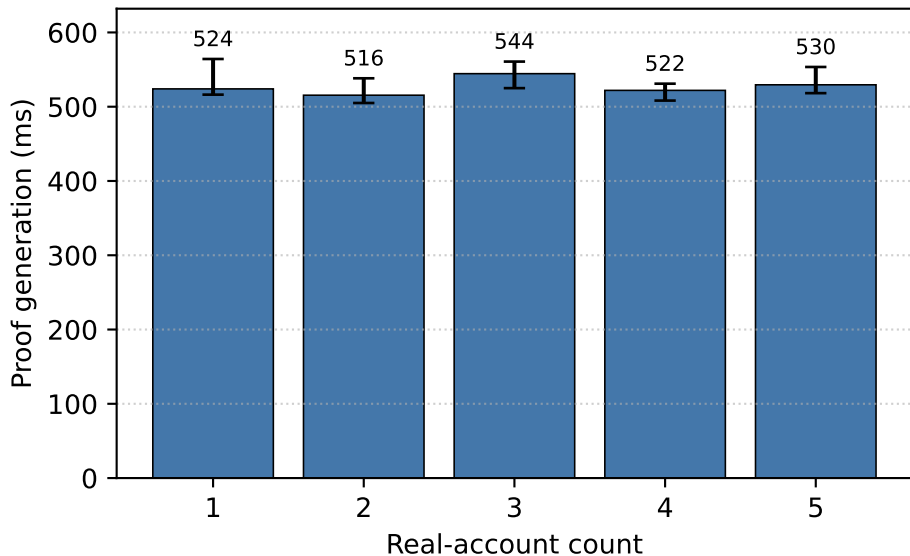
Proof generation time (median with IQR, n = 30)
