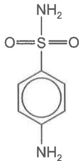
sulfanilamide
