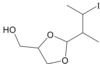
iodinated glycerol
