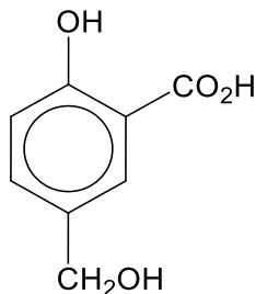
2-hydroxy-5-(hydroxymethyl)benzoic acid
