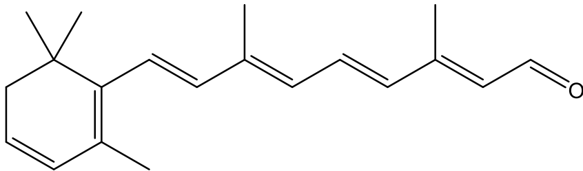
retinal
