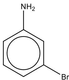
3-bromophenylamine
