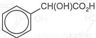
mandelic acid
