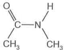
N-methylethanamide
