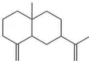
\beta -selinene
