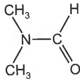
dimethyl formamide
