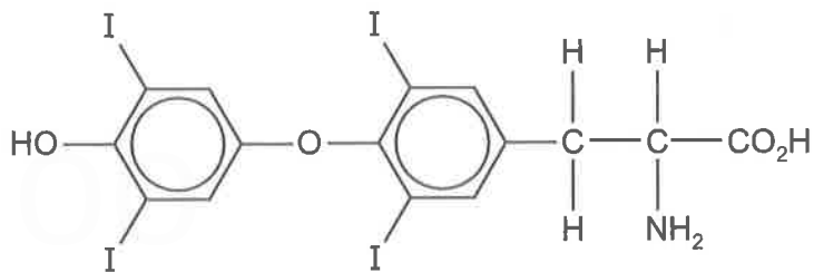
thyroxine
