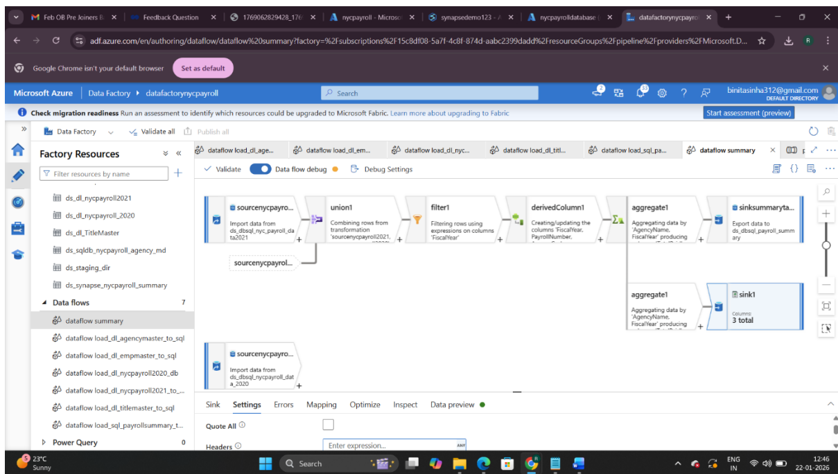
screenshot of aggregate dataflow in Data Factory
