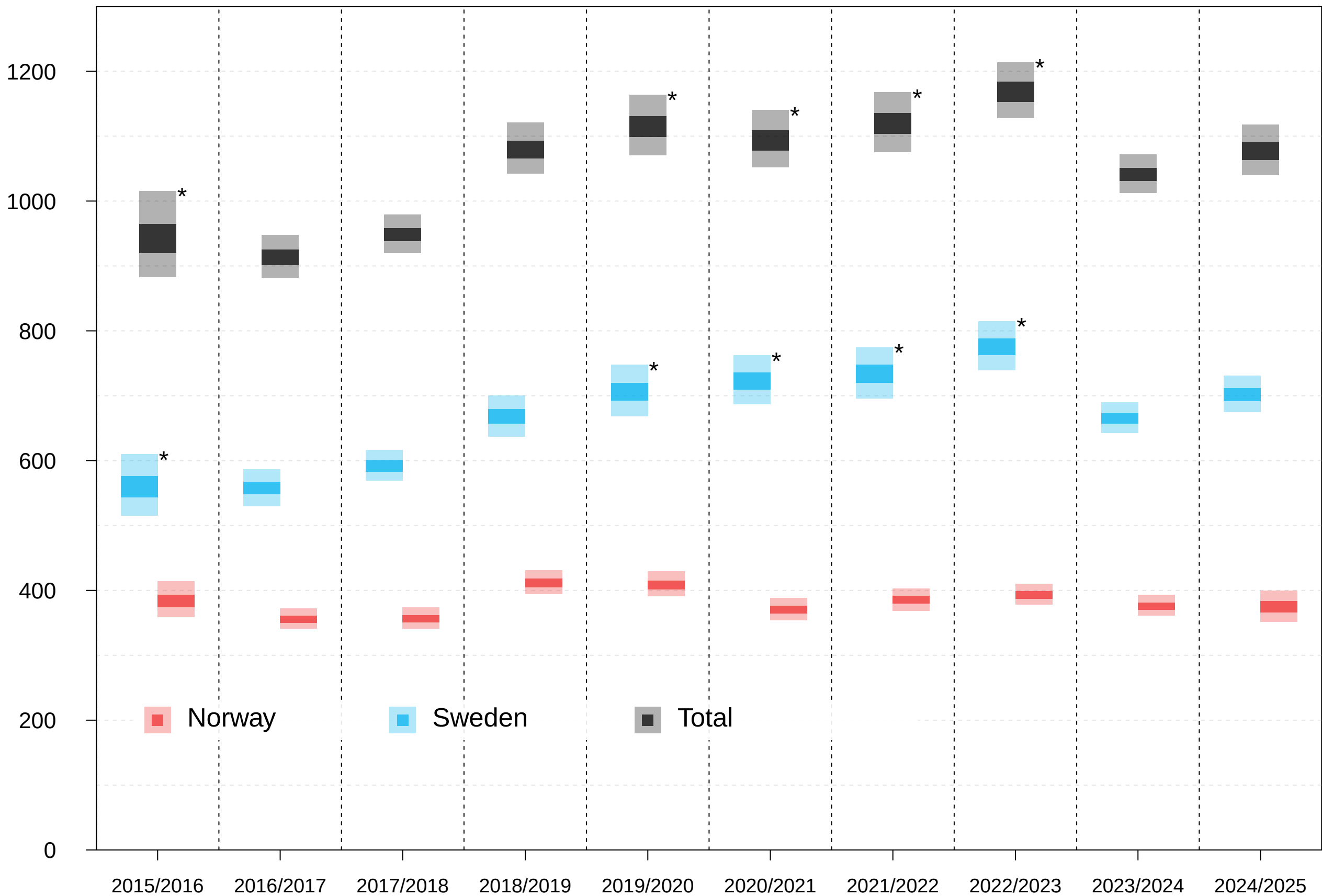
Estimated number of wolverines
