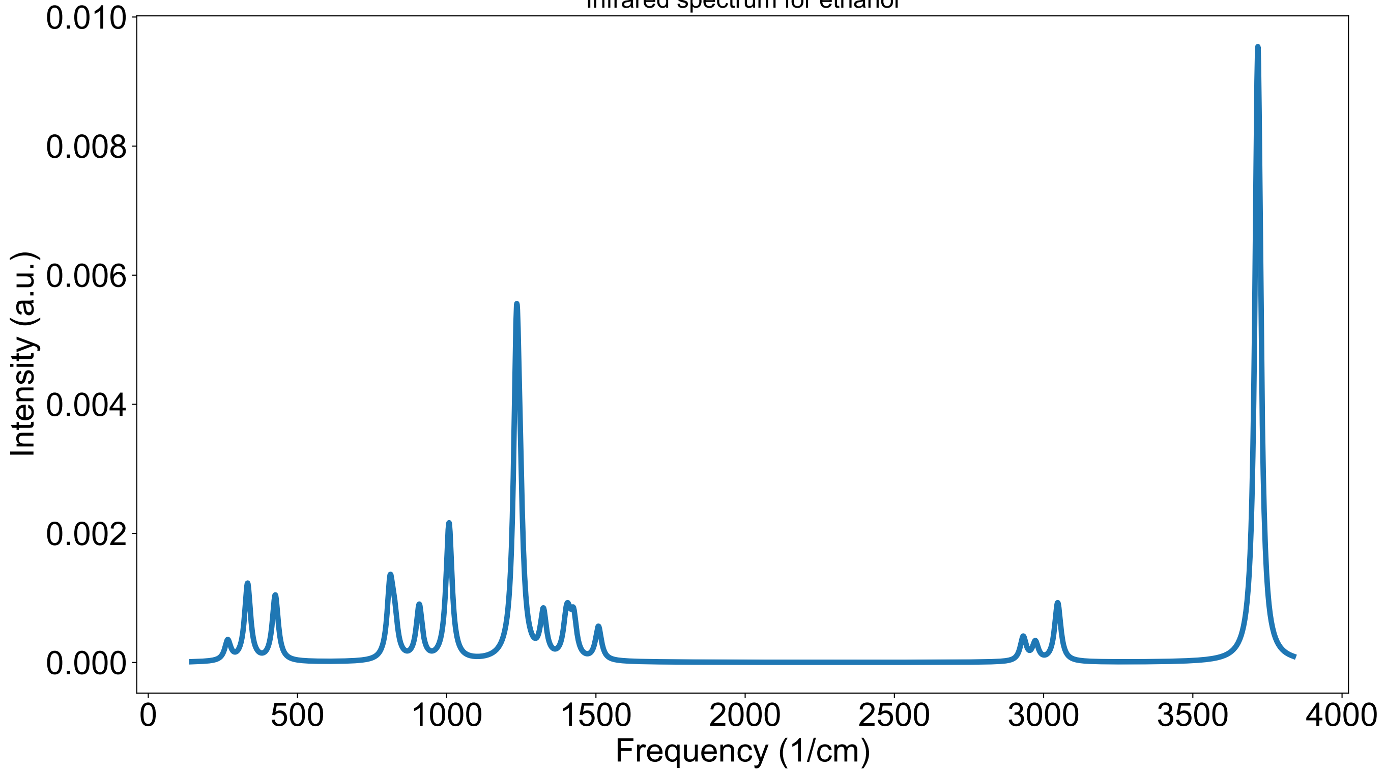
Infrared spectrum for ethanol
