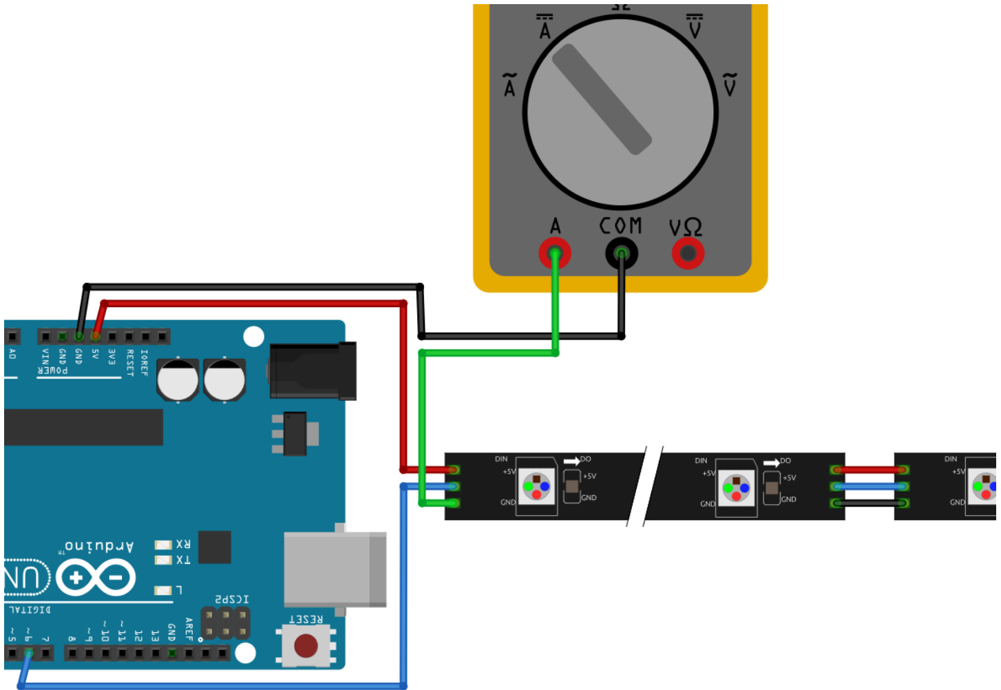
Figure 10: Koppla multimetern i kretsen
