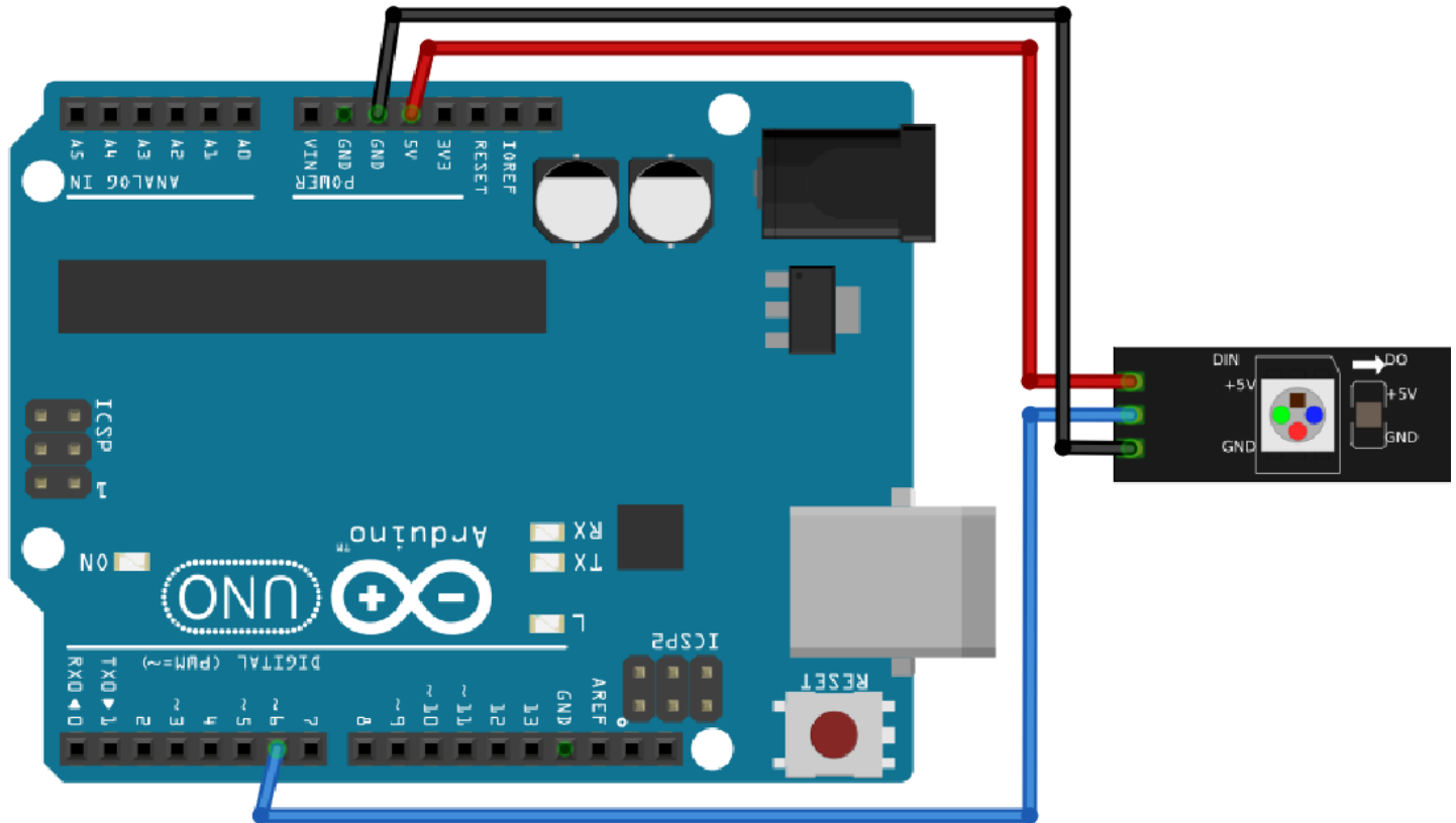
Figure 6: Krets 31.2
