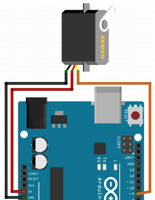
Figure 12: Anslut servomotor
