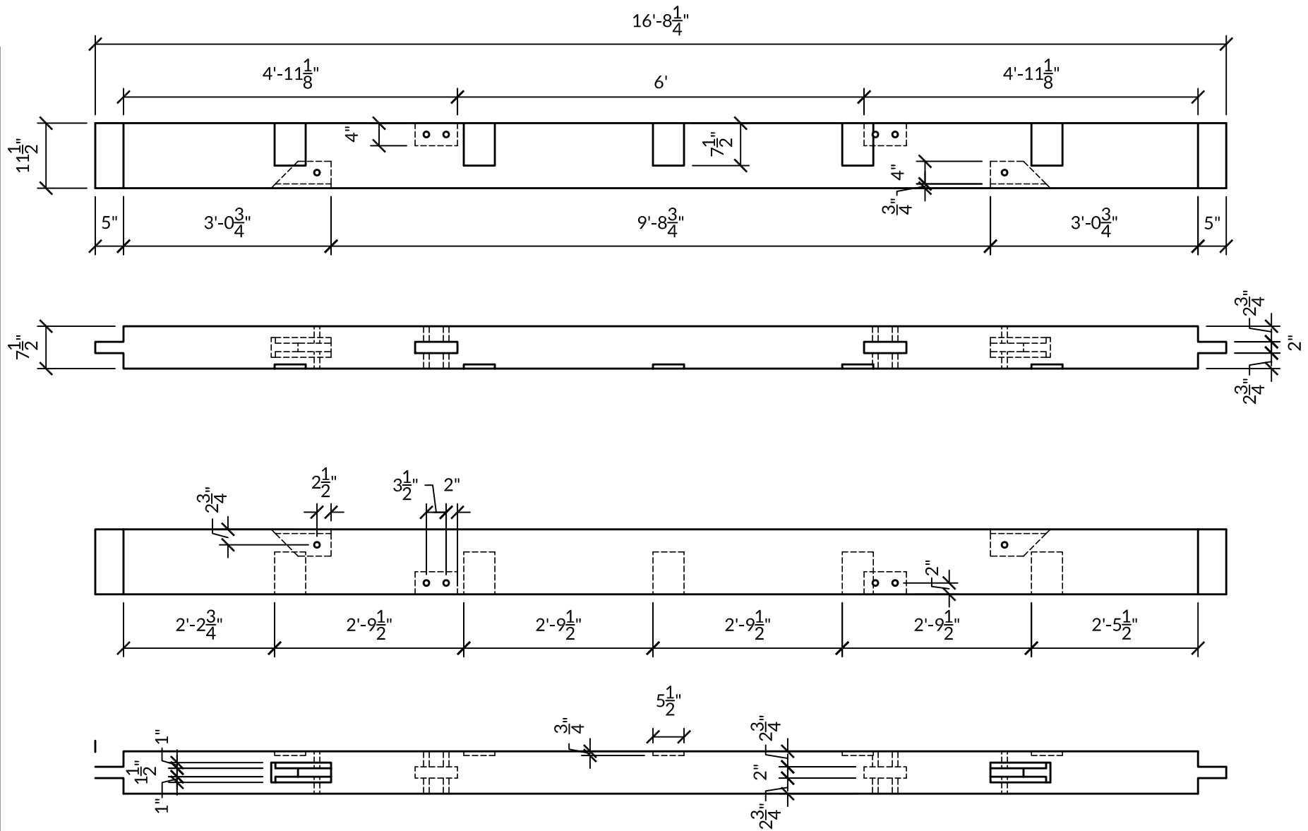
Grid Line 1 Girt Beam Qty: 1
