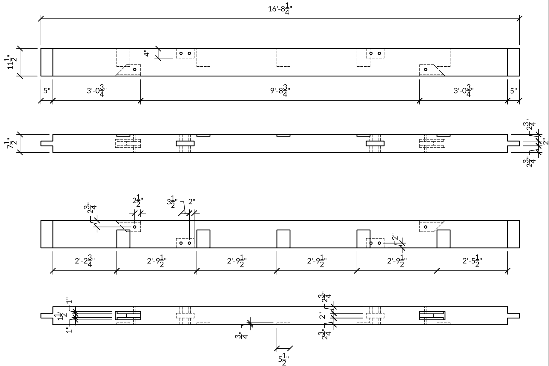
Grid Line 2 Girt Beam Qty: 1
