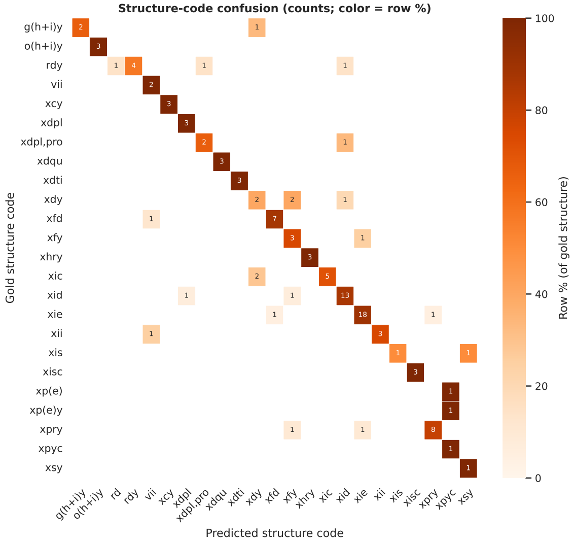
Fig. 12: Structure-code confusion matrix (Run 6).
