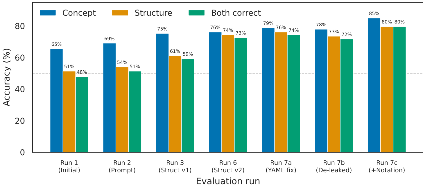
Assertion stage accuracy across prompt-engineering runs
