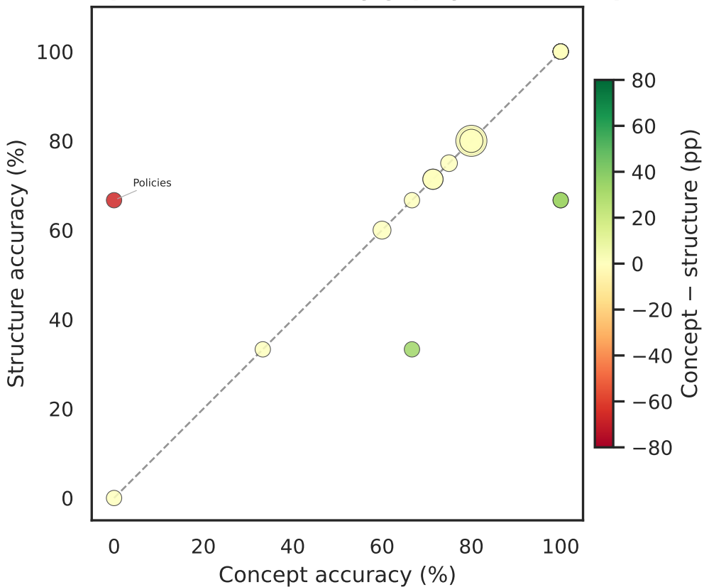
Concept-structure accuracy gap by basic concept
