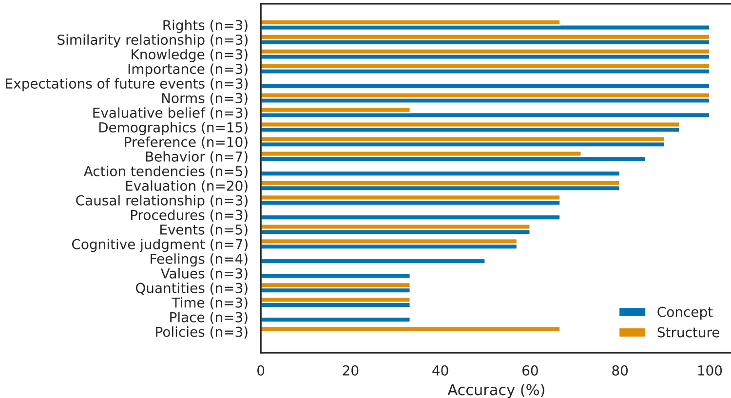
Per-concept accuracy (gold concept labels)
