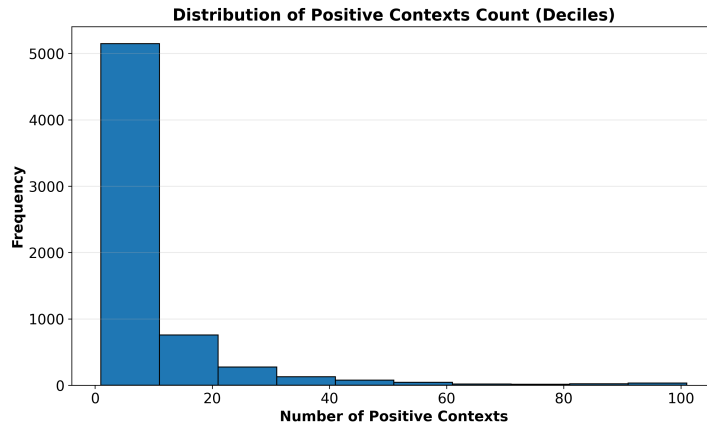
Figure 1: Distribution of annotated correct passage counts per query for SEAL on the NQ dataset.
