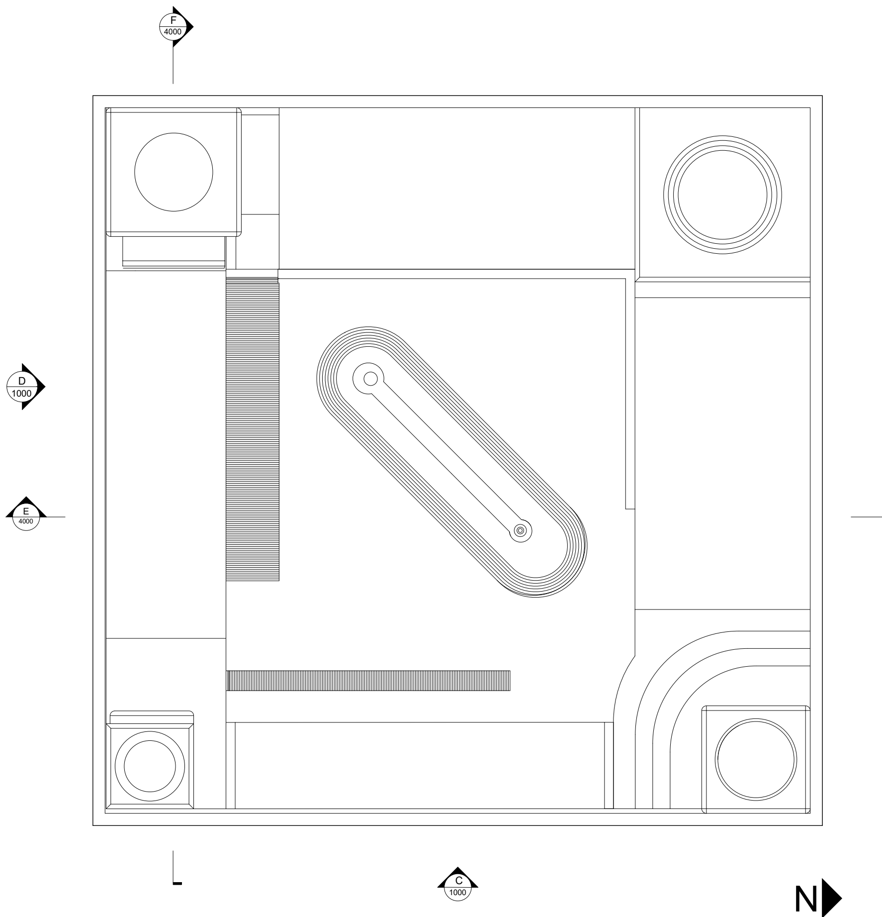
A FIRST FLOOR PLAN
