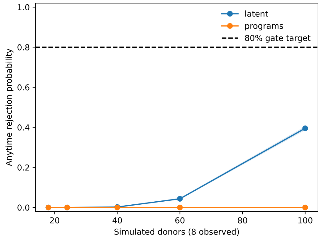
Frozen association critic · fails power target
