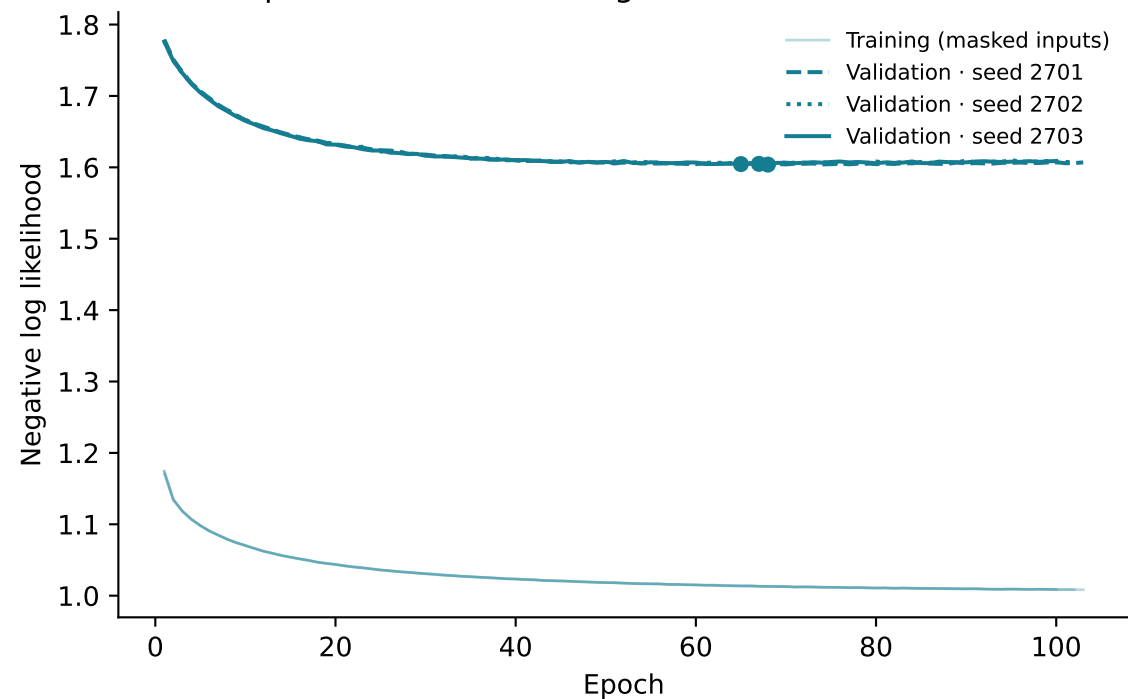
Fibroblast · negative-binomial encoder
