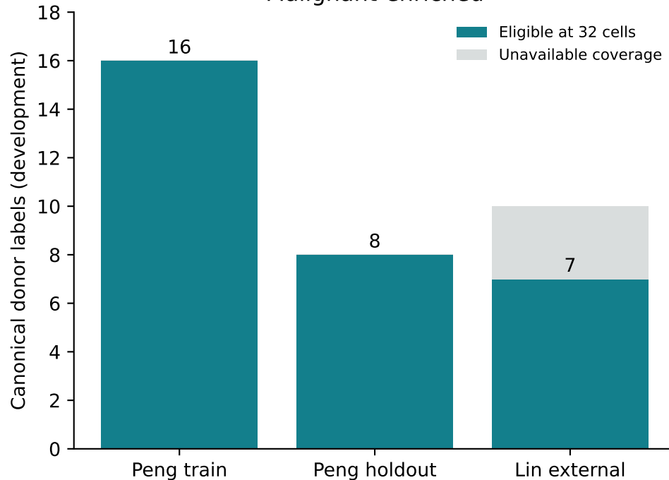
Malignant-enriched
