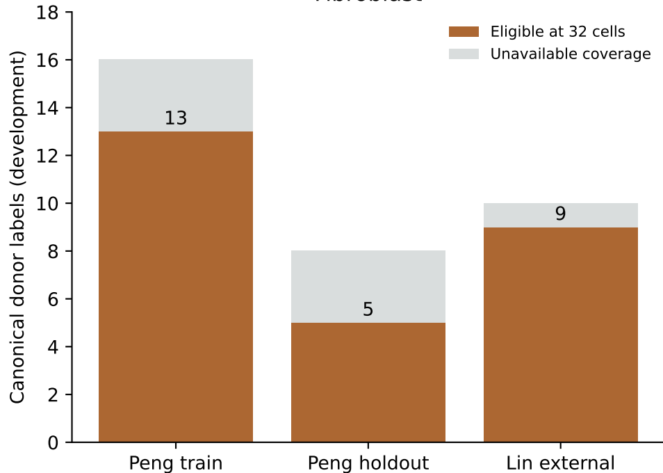
Fibroblast
