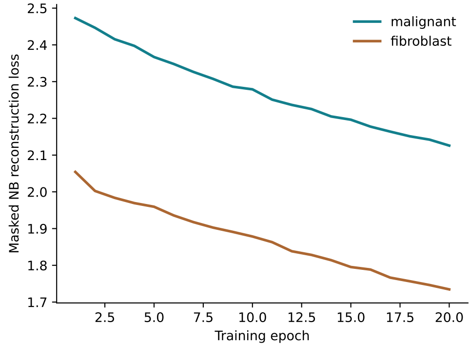
Real count-model training
