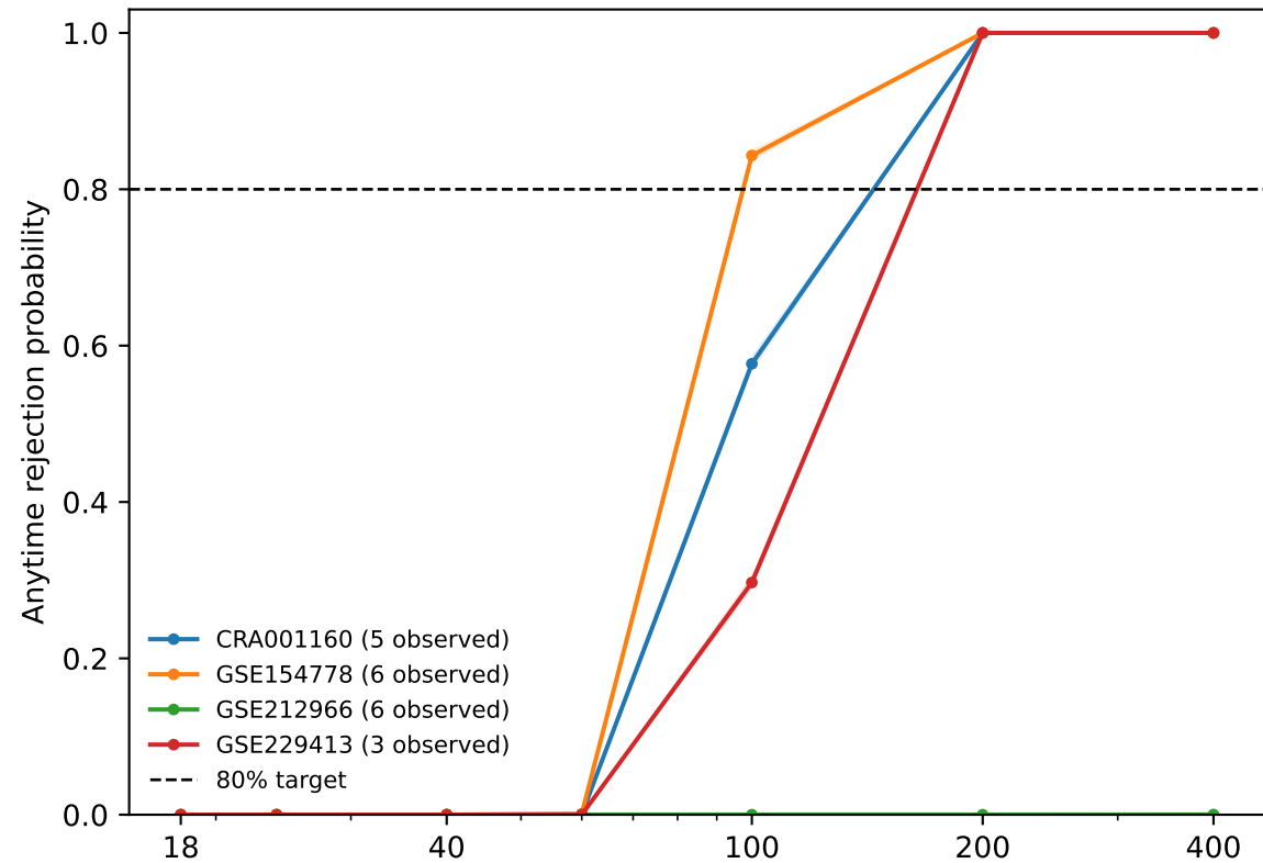
cca-rbf
