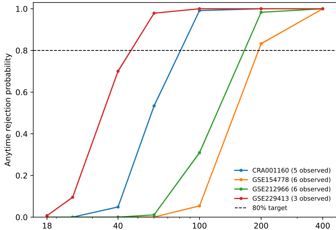
native-growth
