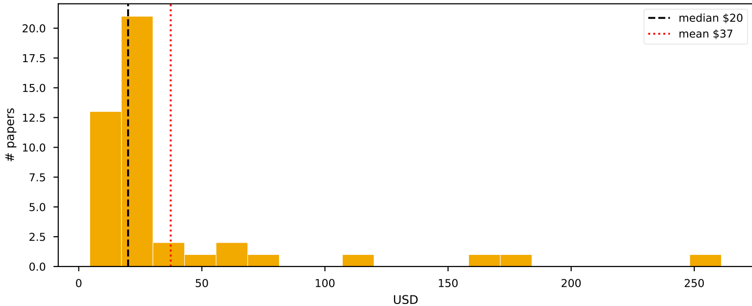
Cost per replication (tokens + GPU + CPU)
