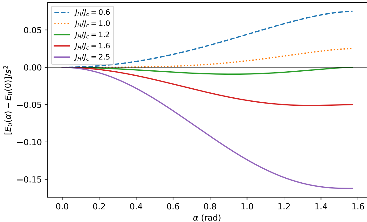
Mean-field energy functional (paper eq. 16)
