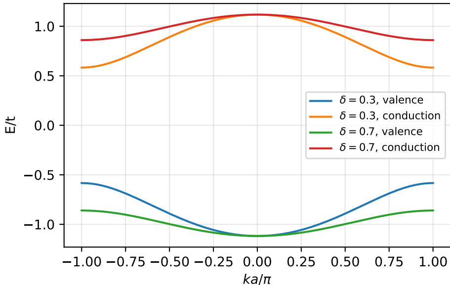
Rice-Mele bands ( \Delta/t = 0.5 )
