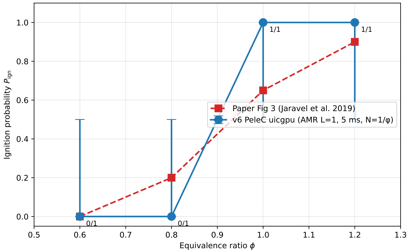
Ignition probability vs \phi — uicgpu v6 sweep (AMR L=1, 5 ms)
